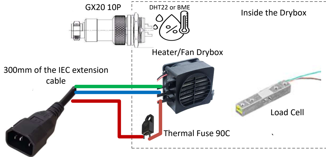
Connections inside the Dry Box GX20
